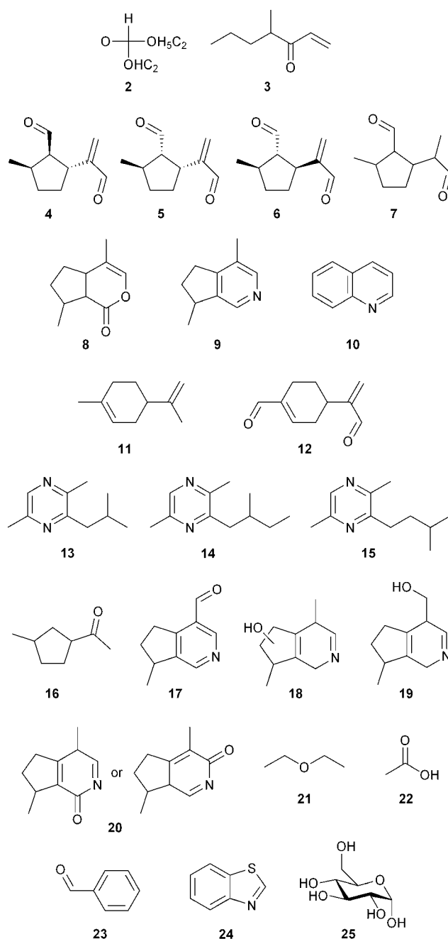
Fig. 5 Compounds from the defense glands of phasmids.
